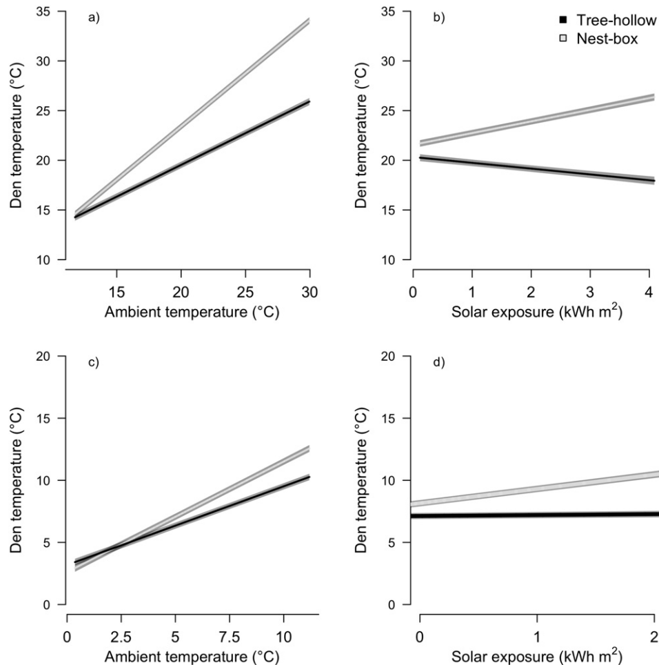
Fig. 2. The modeled fixed-effects of ambient temperature (a, c) and solar exposure (b, d) on mean daytime temperatures of tree-hollows and nest-boxes during summer (a, b) and winter (c, d) in the Strathbogie Ranges, Victoria, (holding other variables at the mean value). Grey bars represent 95% confidence intervals. See Table 1 for statistical analyses.
