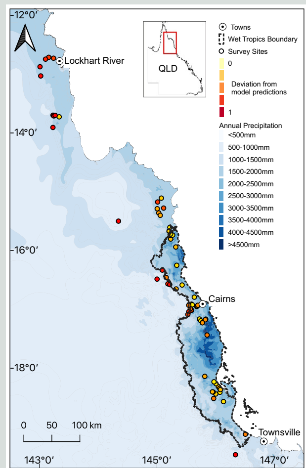
Figure 1: The location of the watergum survey sites in Queensland and the average annual rainfall of the area. Areas of high annual rainfall are indicated by dark shading. The colour gradient within the survey points represents the accuracy of the myrtle rust model, with lighter shading indicating greater similarity between the model predictions and field observations.
