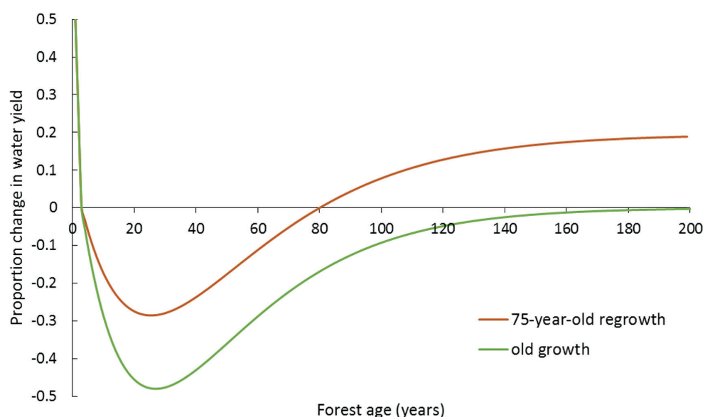
Figure 4.2. Reduction in water yield in montane ash forest estimated as a proportion of the pre-disturbance amount in regrowth and old growth forest.
