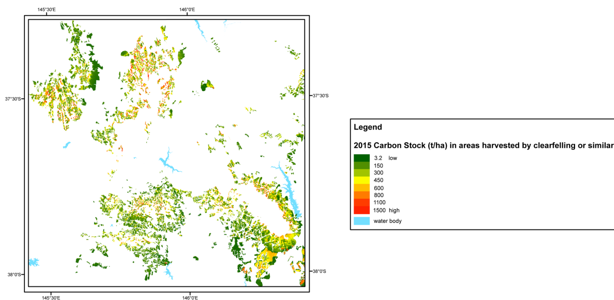
Figure 5.3. Carbon stock ( \text{tC ha}^{-1} ) in 2015 in the areas logged previously in all forest types by stand-replacing activities.
